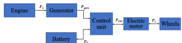
Figure 1. Series HEV structure
